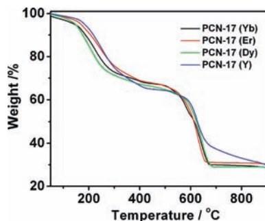
Figure 4. TGA profiles of PCN-17 (Dy, Er, Y, Yb).
