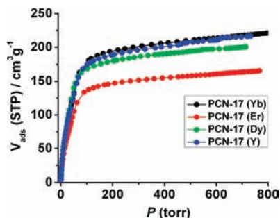
Figure 2. CO 2 adsorption isotherms of PCN-17 (Dy, Er, Y, Yb) at 195 K.
