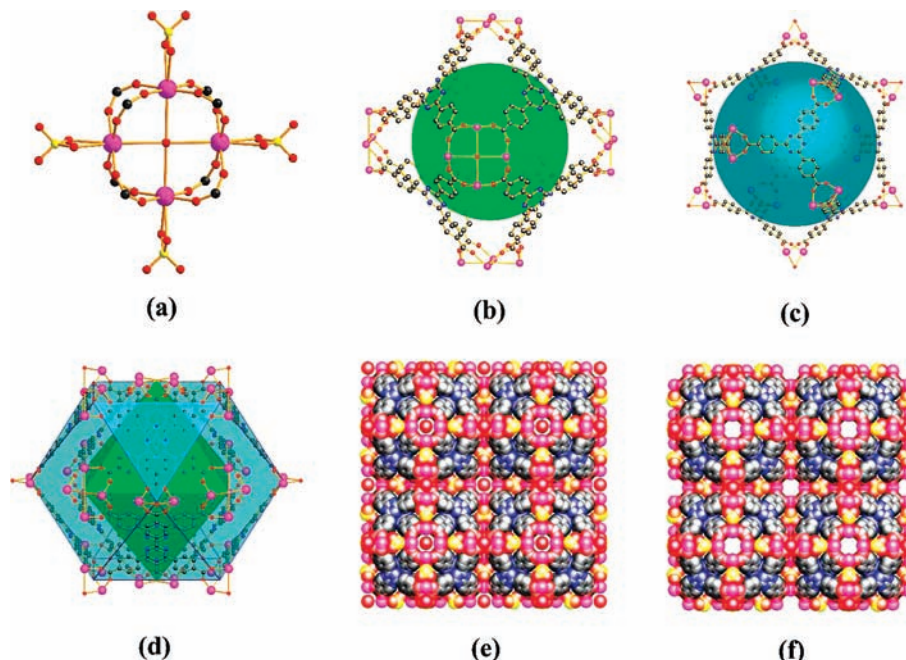
Figure 1. Structures of PCN-17 (Dy, Er, Y, Yb): (a) \text{Ln}_4(\mu_4\text{-H}_2\text{O}) SBUs; (b) octahedral cage; (c) cuboctahedral cage; (d) an octahedral cage enclosed by another network; (e) space-filling packing of unactivated sulfate-bridging doubly interpenetrated (8,3)-connected net (viewed from (1 0 0) direction); (f) space-filling packing of activated sulfate-bridging doubly interpenetrated (8,3)-connected net with open tiny pores resulted from the removal of the \mu_4\text{-H}_2\text{O} of the SBUs (viewed from (1 0 0) direction). (Pink, Ln (Ln = Dy, Er, Y, Yb); gray, carbon; red, oxygen; yellow, sulfur).
