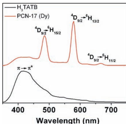
Figure 5. Room temperature solid-state photoluminescence spectra of H 3 TATB and PCN-17 (Dy).
