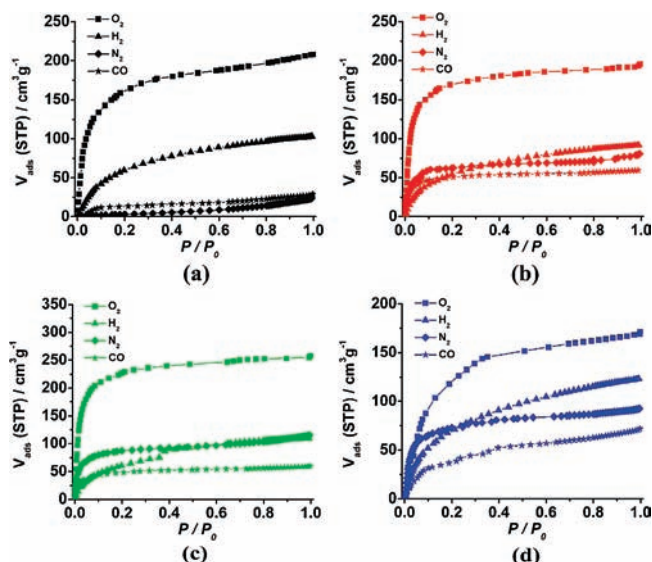
Figure 3. O 2 , H 2 , N 2 , and CO adsorption isotherms of (a) PCN-17 (Yb); (b) PCN-17 (Er); (c) PCN-17 (Dy); (d) PCN-17 (Y) at 77 K.
